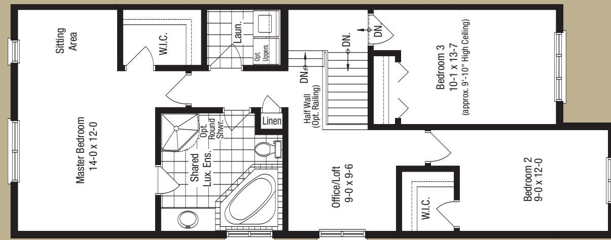
OPTION #2 THE MAGNOLIA Shared Luxury Ensuite Second Floor 1005 sq.ft.
