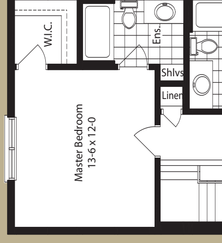
OPTION #1 ELDERBERRY (Left) Master Bedroom Ensuite
