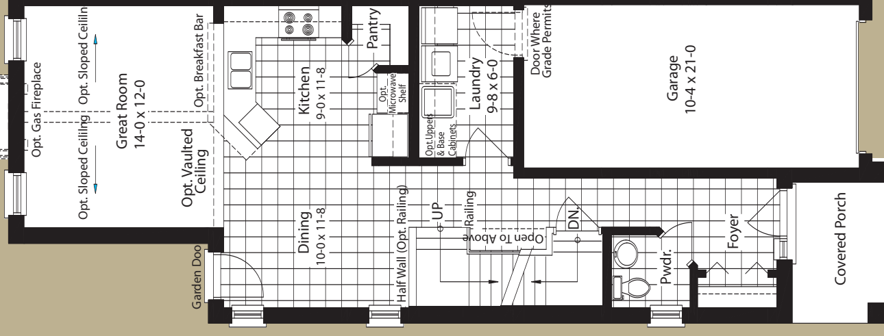
ELDERBERRY (Left) First Floor Plan-742sq.ft.
